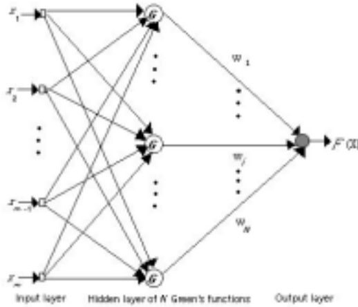
Figure 4: Regularization Network
