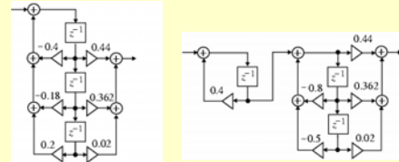
Direct form II
