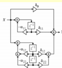
Parallel form II
