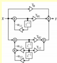
Parallel form I
