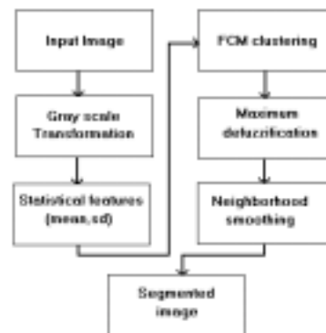
Figure 9: Segmentation method
