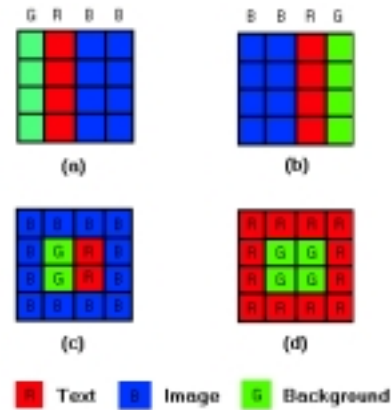
Figure 7: Neighborhood Smoothing
