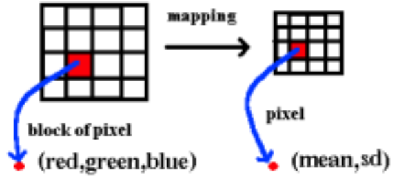
Figure 2: Color-to-gray mapping
