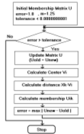
Figure 6: The FCM Classification Process
