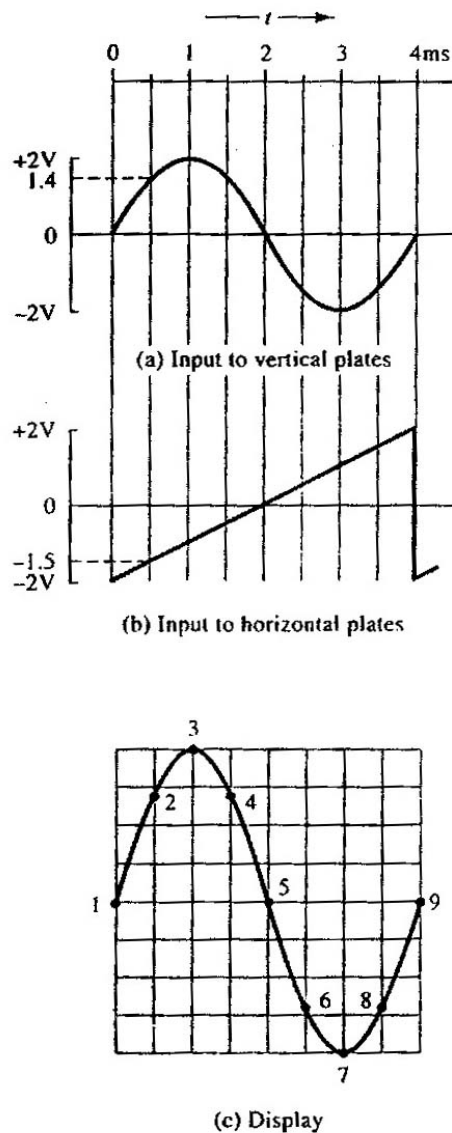
Fig. 3 The synchronization of a sine wave with a sawtooth wave resulting in a graphical display on the screen.
