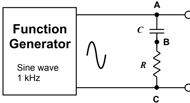
Fig.4 Circuit used in the experiment
