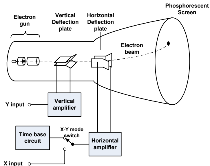
Fig. 1 Simple oscilloscope construction.
